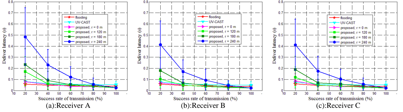
Fig. 9. The deliver latency under each protocol with different transmission conditions observed at the receiver A, B and C, respectively. (a) Observed at receiver A. (b) Observed at receiver B. (c) Observed at receiver C.
